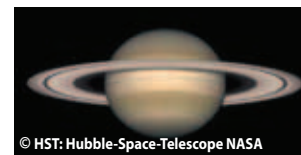
© HST: Hubble-Space-Telescope NASA
